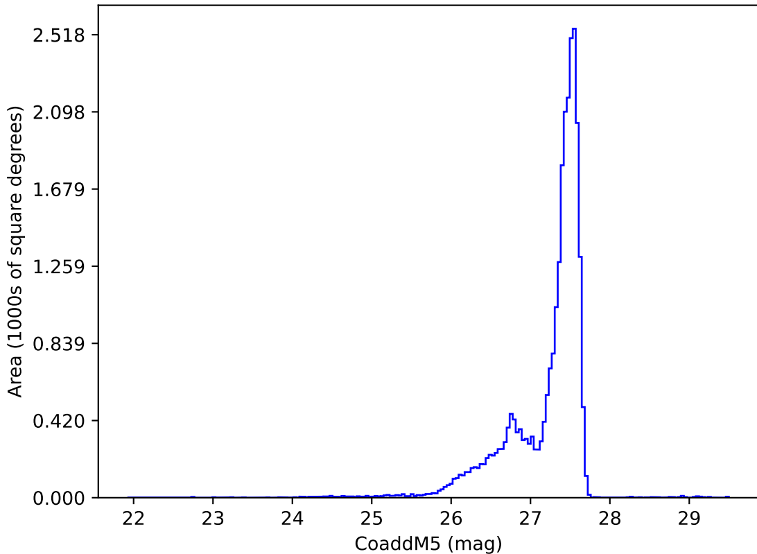
internal_u_expt30_nscale0.9v3.4_10yrs : CoaddM5
