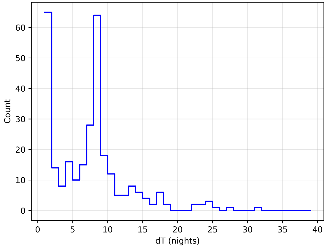
internal_u_expt30_nscale0.9v3.4_10yrs all bands: DD:XMM_LSS Delta Nights Histogram
