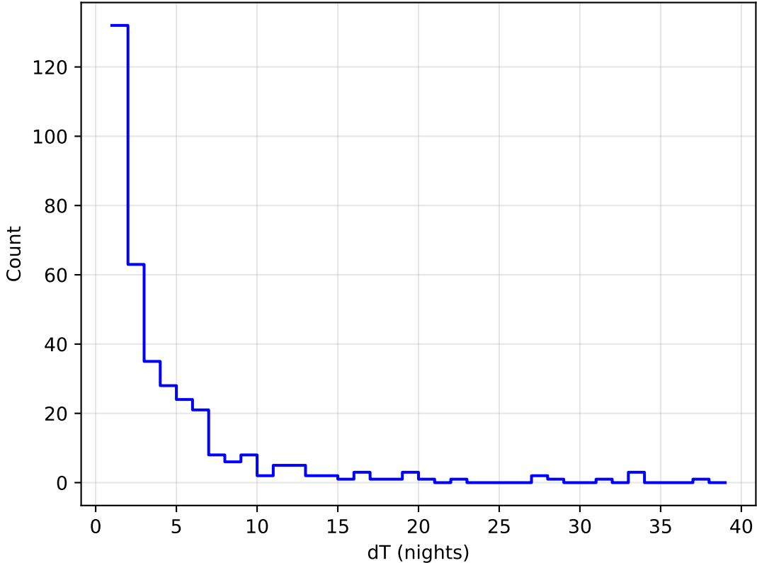
internal_u_expt30_nscale0.9v3.4_10yrs all bands: DD:WFD Delta Nights Histogram
