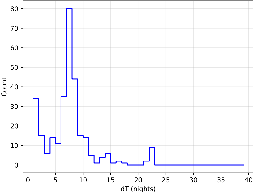
internal_u_expt30_nscale0.9v3.4_10yrs all bands: DD:EDFS Delta Nights Histogram
