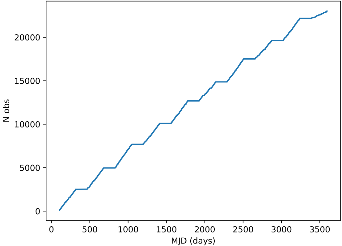
internal_u_expt30_nscale0.9v3.4_10yrs all bands: DD:EDFS Cumulative NVisits
