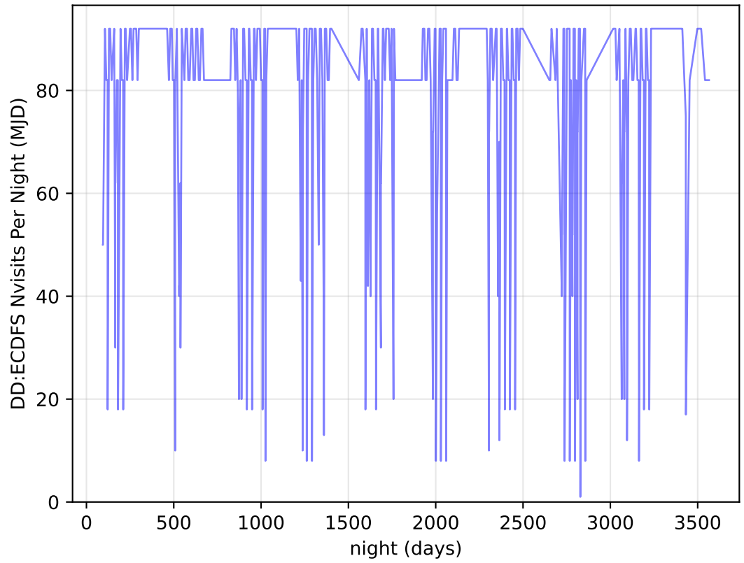
internal_u_expt30_nscale0.9v3.4_10yrs all bands: DD:ECDFS Nvisits Per Night
