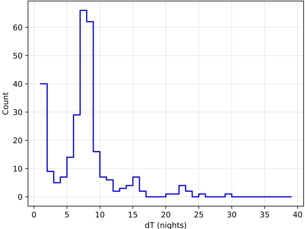
internal_u_expt30_nscale0.9v3.4_10yrs all bands: DD:ECDFS Delta Nights Histogram
