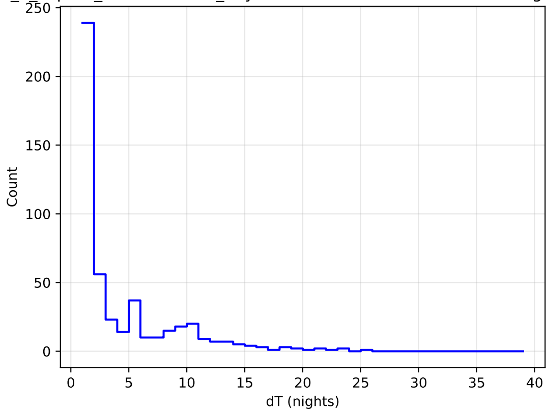
internal_u_expt30_nscale0.9v3.4_10yrs all bands: DD: COSMOS Delta Nights Histogram
