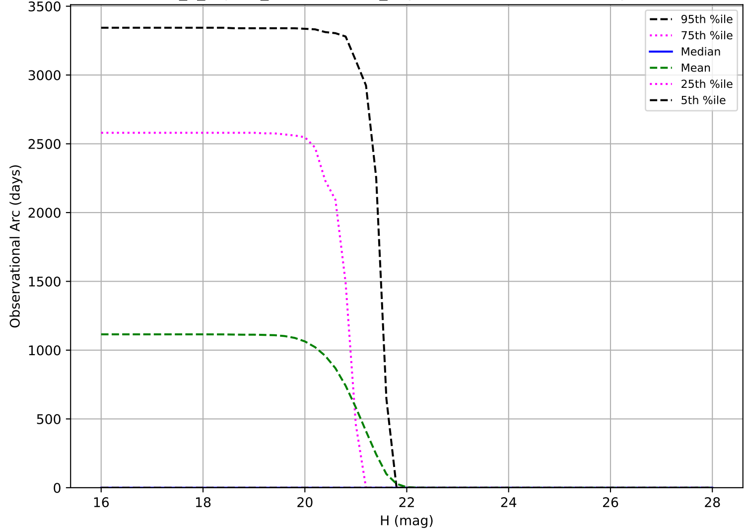
internal_u_expt27_nscale1.5v3.4_10yrs: Observational Arc Length Vatira
