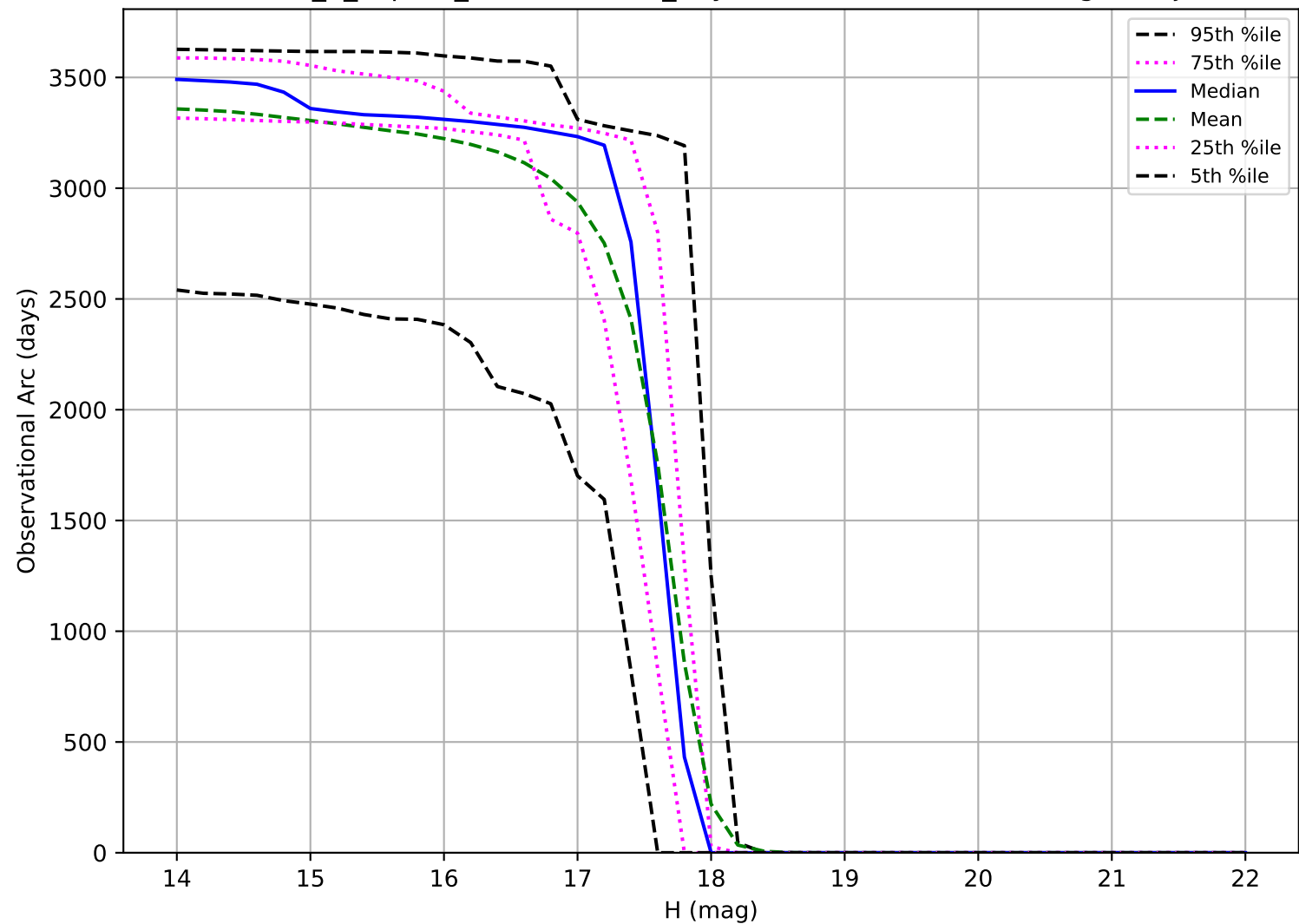
internal_u_expt27_nscale1.5v3.4_10yrs: Observational Arc Length Trojan
