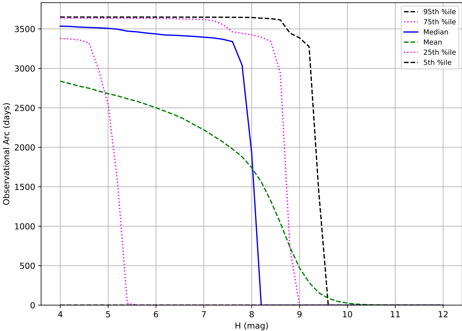
internal_u_expt27_nscale1.5v3.4_10yrs: Observational Arc Length TNO
