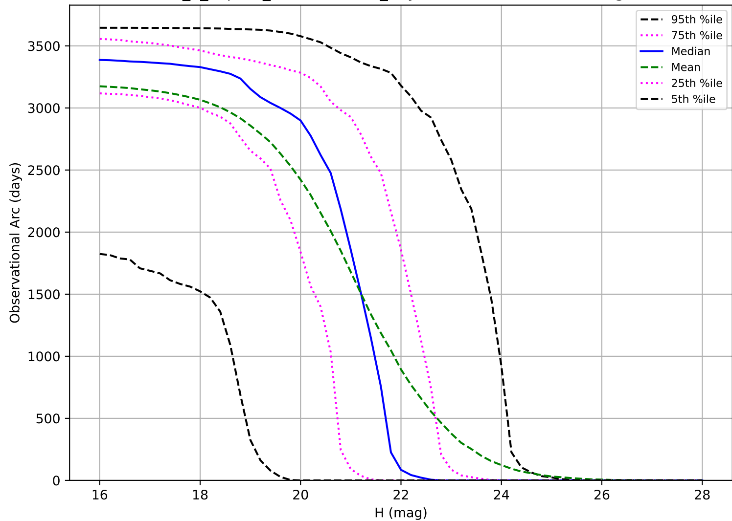
internal_u_expt27_nscales1.5v3.4_10yrs: Observational Arc Length NEO
