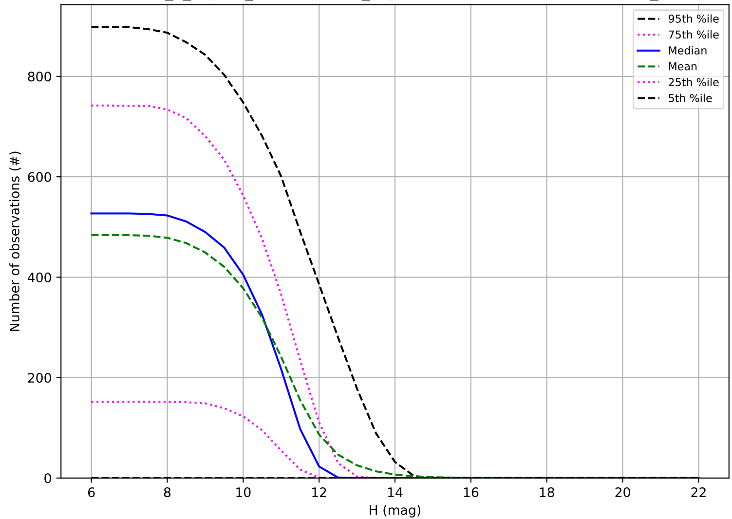
internal_u_expt27_nscale1.5v3.4_10yrs: Number of observations OCC_r20
