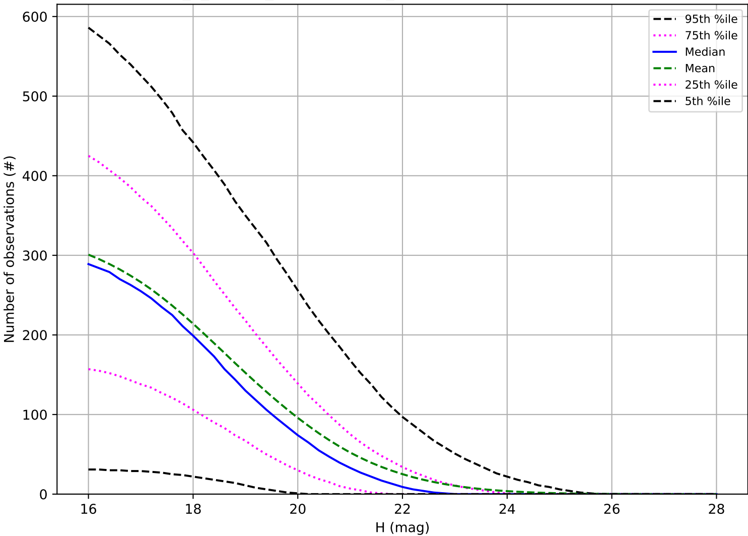
internal_u_expt27_nscale1.5v3.4_10yrs: Number of observations NEO
