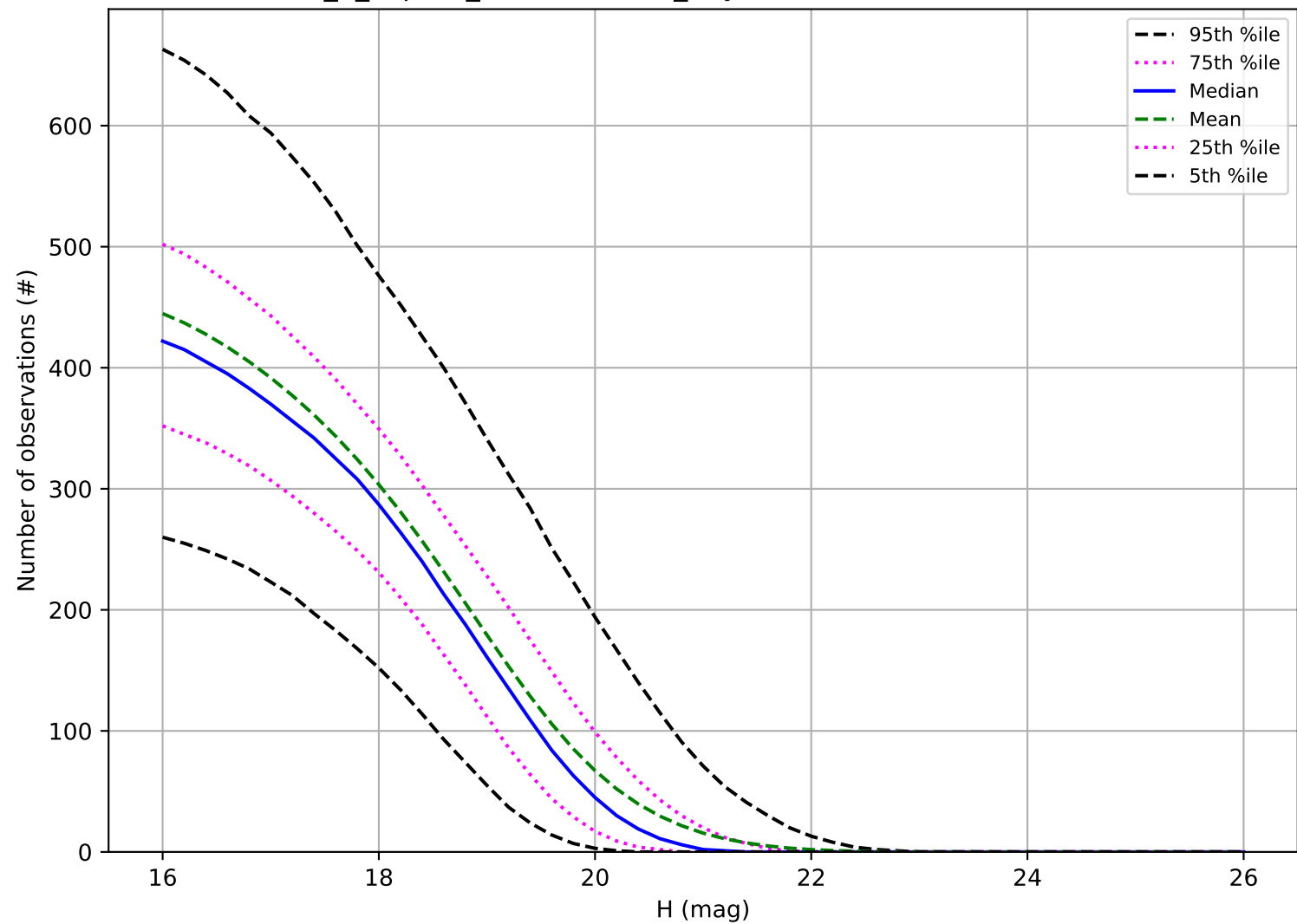
internal_u_expt27_nscale1.5v3.4_10yrs: Number of observations MBA
