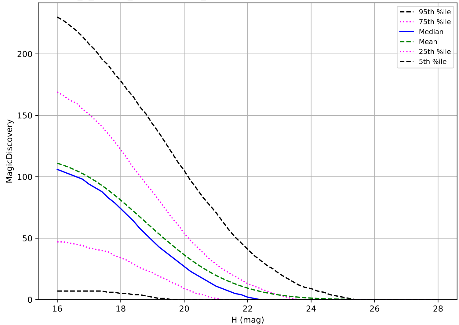
internal_u_expt27_nscale1.5v3.4_10yrs: PHA 6 detections in 60 nights detection loss
