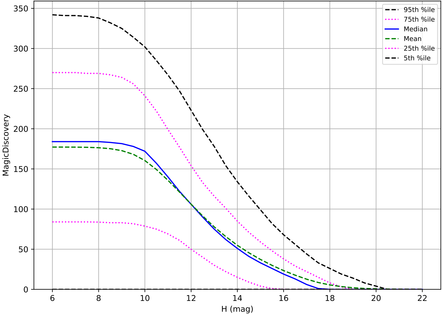
internal_u_expt27_nscale1.5v3.4_10yrs: OCC_r5 6 detections in 60 nights detection loss
