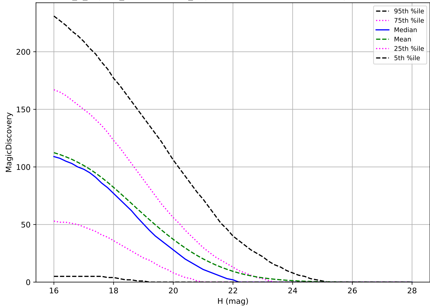
internal_u_expt27_nscale1.5v3.4_10yrs: NEO 6 detections in 60 nights detection loss
