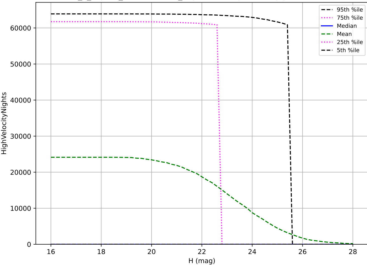
internal_u_expt27_nscale1.5v3.4_10yrs: PHA High velocity pair detection loss
