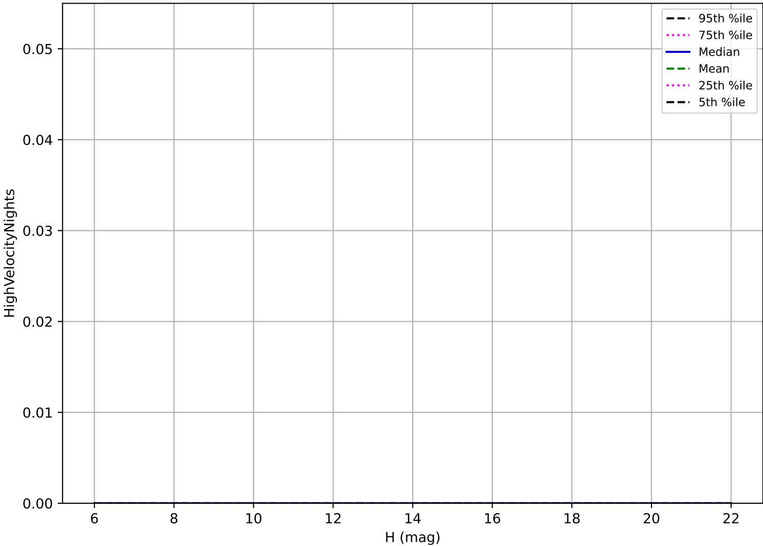
internal_u_expt27_nscale1.5v3.4_10yrs: OCC_r5 High velocity pair detection loss
