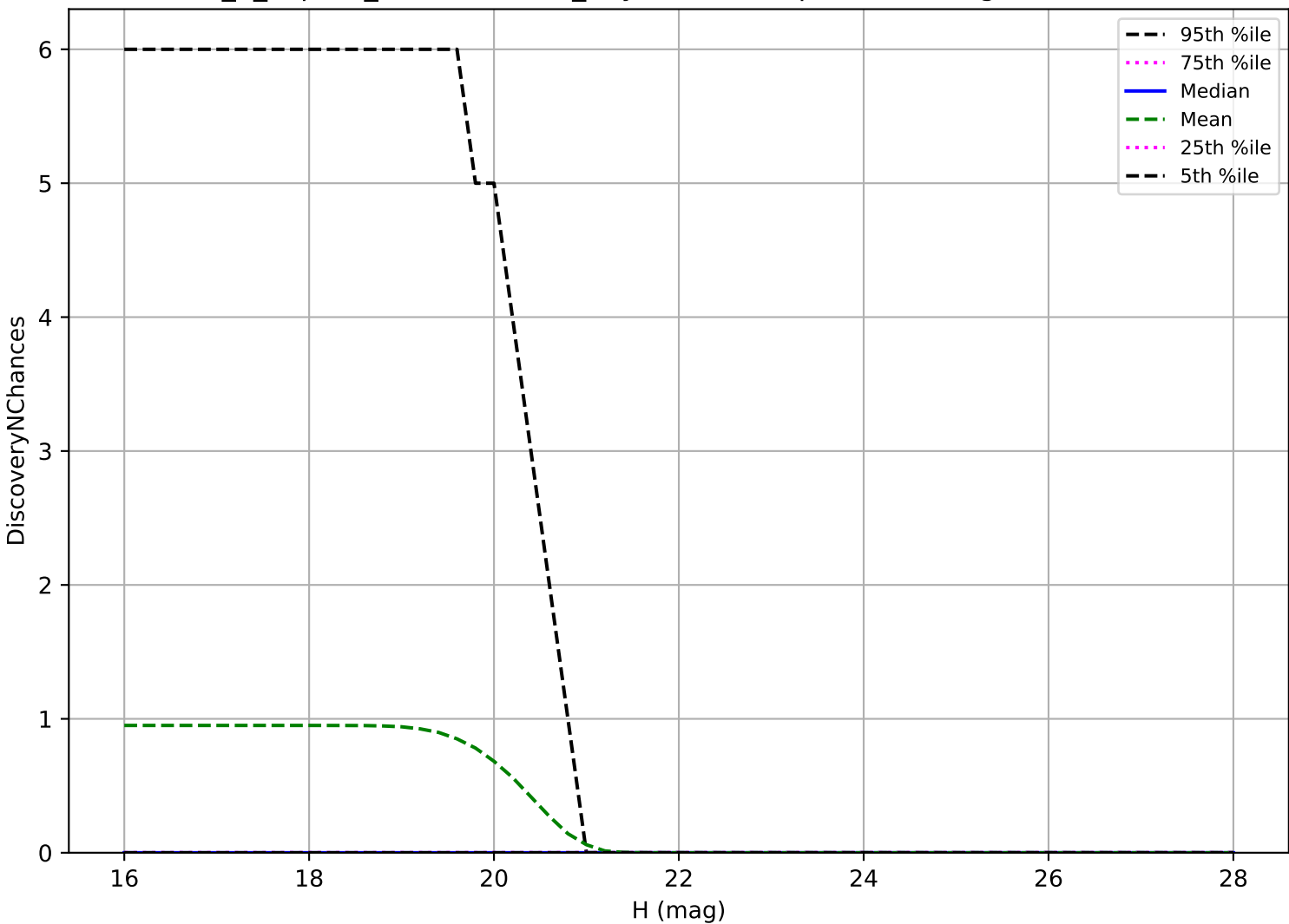
internal_u_expt27_nscale1.5v3.4_10yrs: Vatira 3 pairs in 15 nights detection loss
