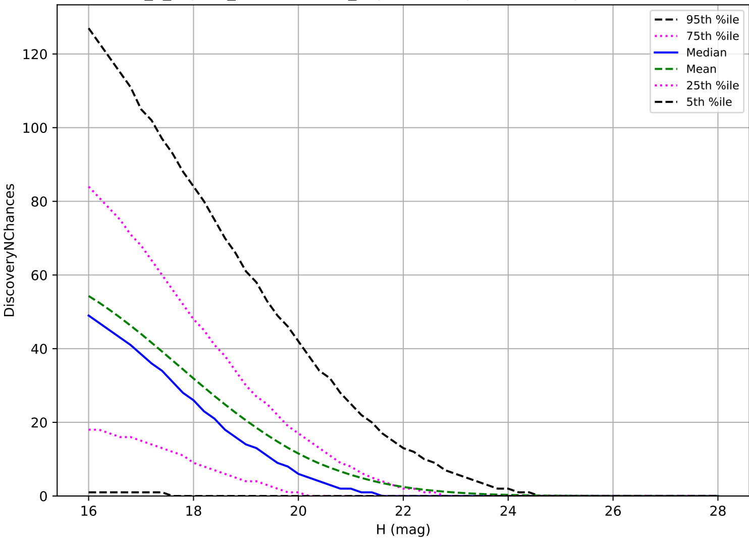
internal_u_expt27_nscale1.5v3.4_10yrs: PHA 3 pairs in 15 nights detection loss
