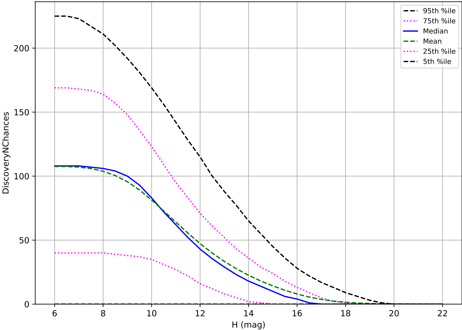
internal_u_expt27_nscale1.5v3.4_10yrs: OCC_r5 3 pairs in 15 nights detection loss
