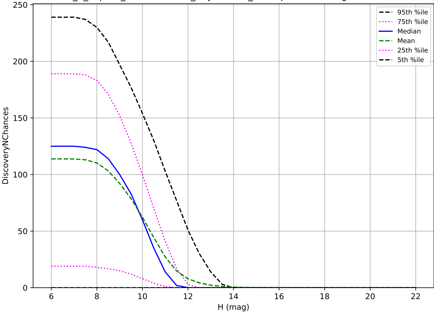
internal_u_expt27_nscale1.5v3.4_10yrs: OCC_r20 3 pairs in 15 nights detection loss
