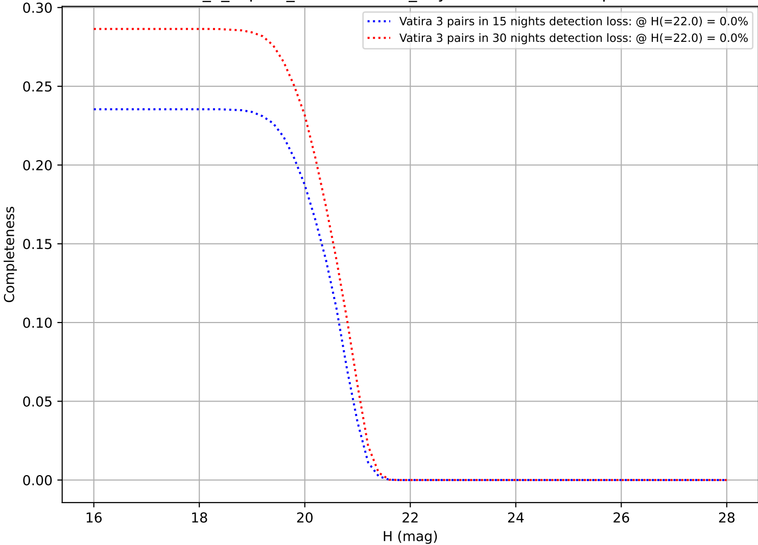
internal_u_expt27_nscales1.5v3.4_10yrs: DifferentialCompleteness
