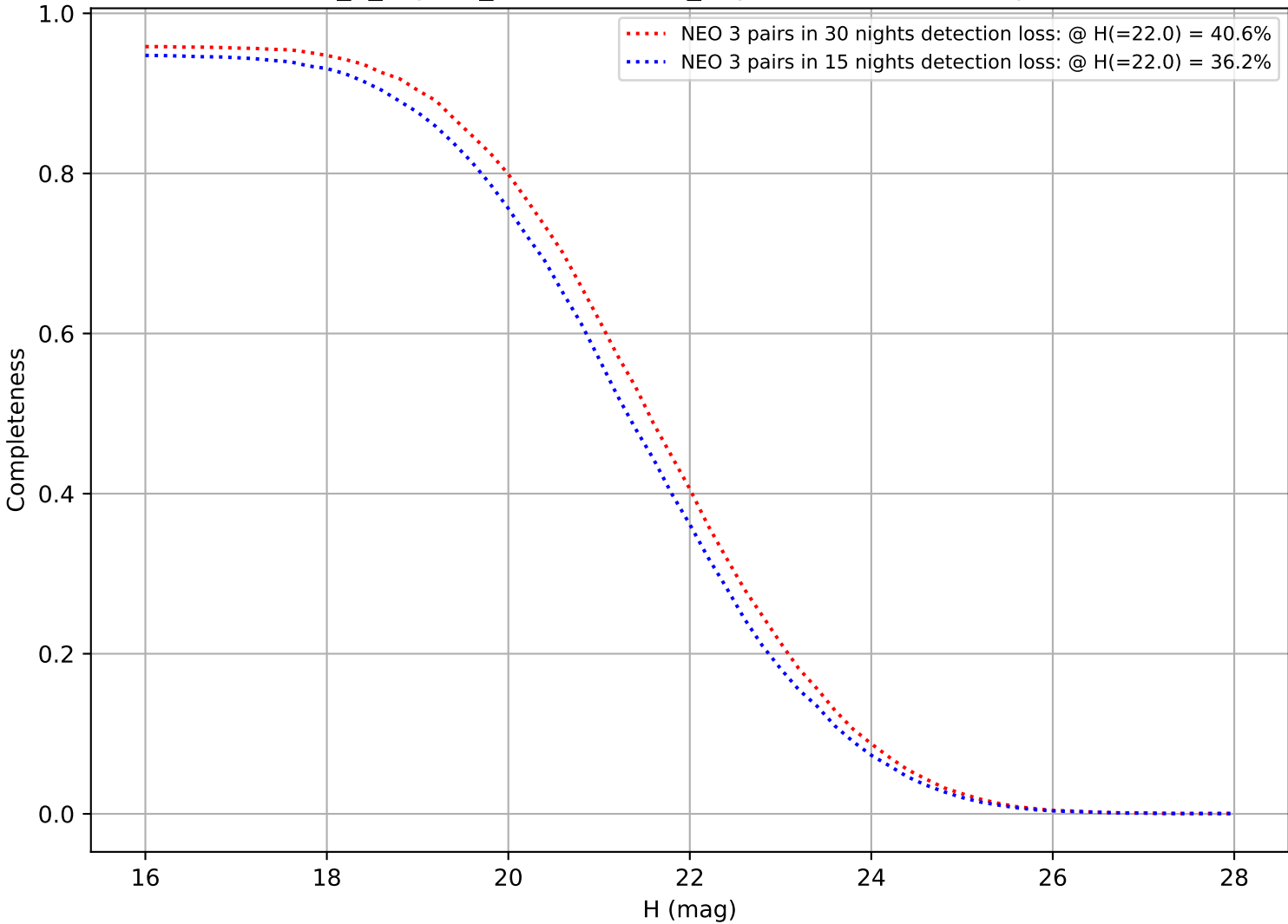
internal_u_expt27_nscale1.5v3.4_10yrs: DifferentialCompleteness
