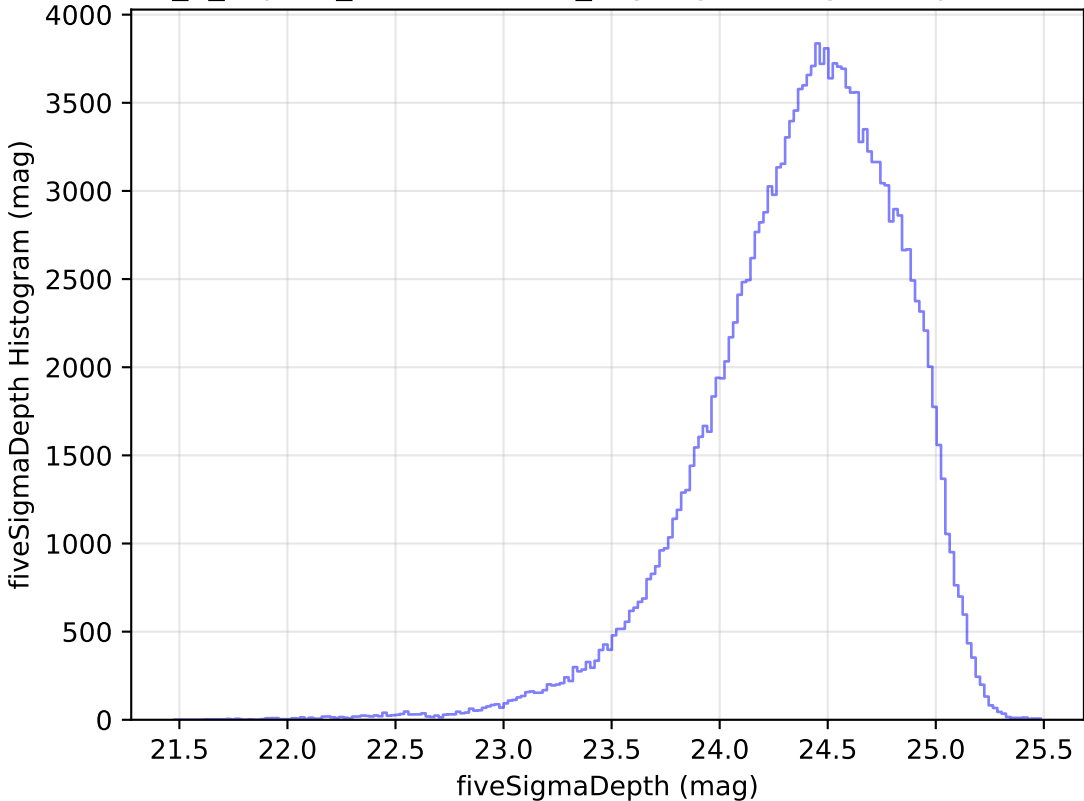
internal_u_expt27_nscale1.5v3.4_10yrs g: fiveSigmaDepth Histogram
