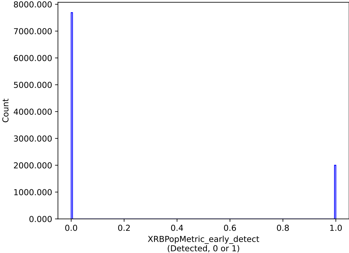
internal_u_expt27_nscale1.5v3.4_10yrs : XRBPoMetric_early_detect
