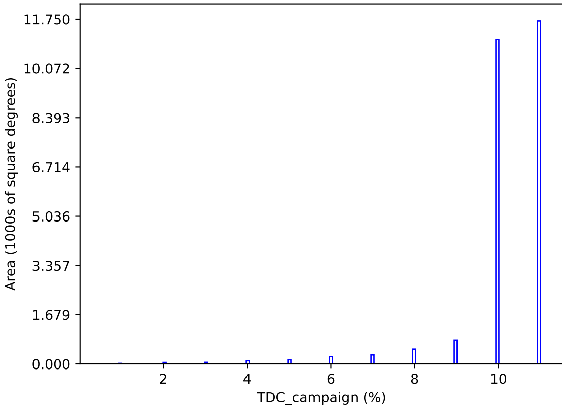
internal_u_expt27_nscale1.5v3.4_10yrs : TDC_campaign
