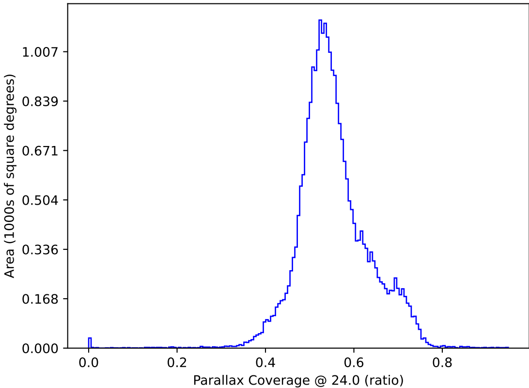
internal_u_expt27_nscale1.5v3.4_10yrs : Parallax Coverage @ 24.0
