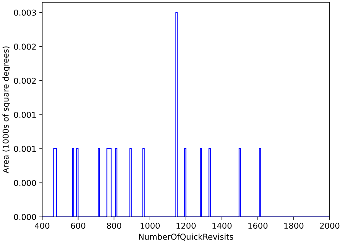
internal_u_expt27_nscale1.5v3.4_10yrs : NumberOfQuickRevisits
