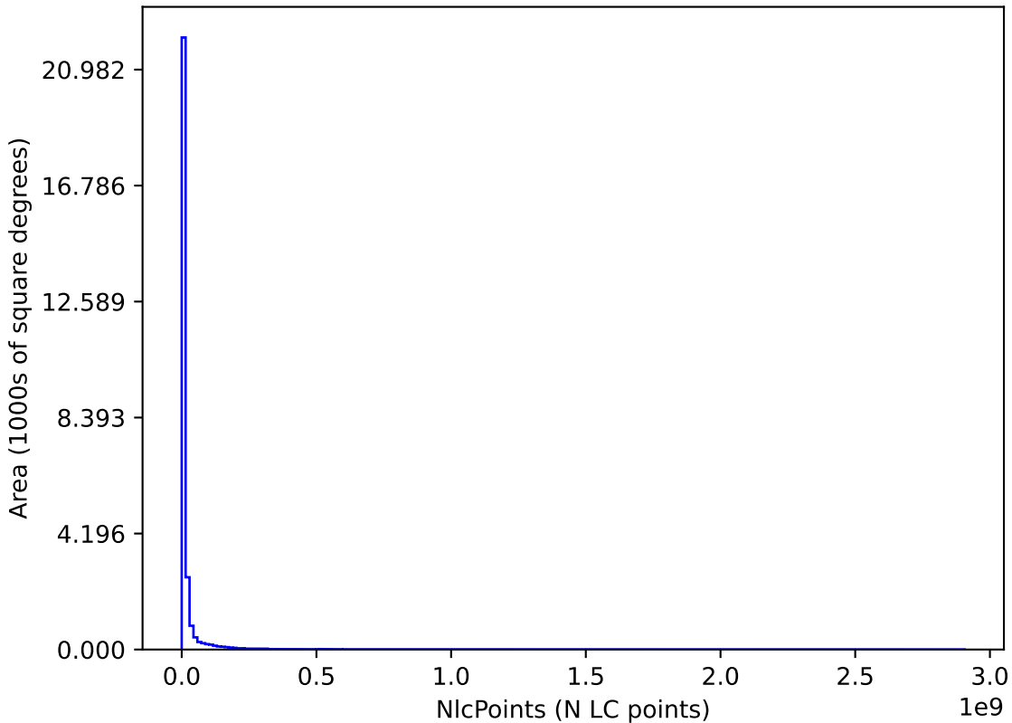
internal_u_expt27_nscale1.5v3.4_10yrs : NlcPoints
