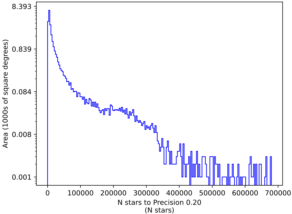
internal_u_expt27_nscale1.5v3.4_10yrs u: N stars to Precision 0.20
