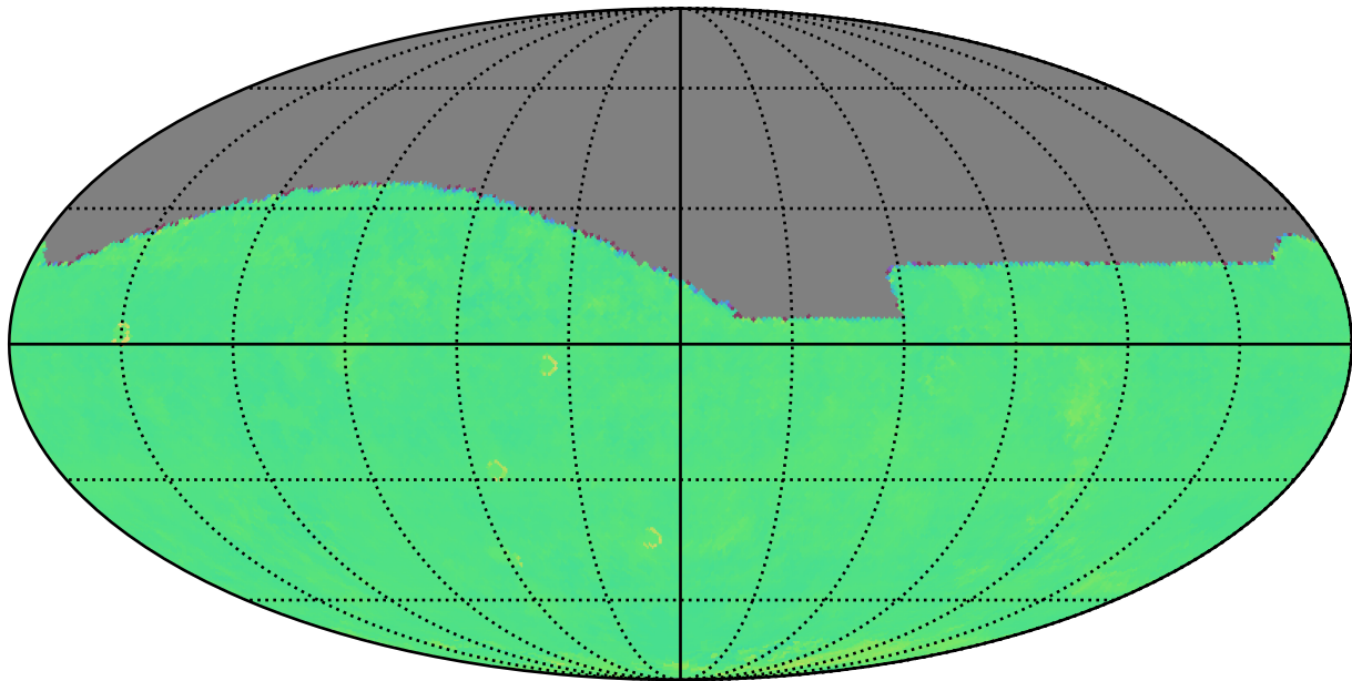
internal_u_expt27_nscale1.5v3.4_10yrs r: Kuiper rotTelPos
