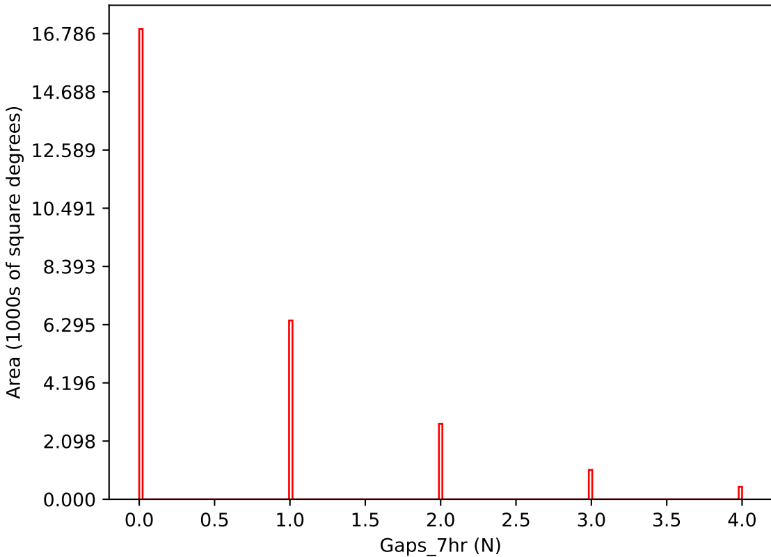
internal_u_expt27_nscale1.5v3.4_10yrs i band: Gaps_7hr
