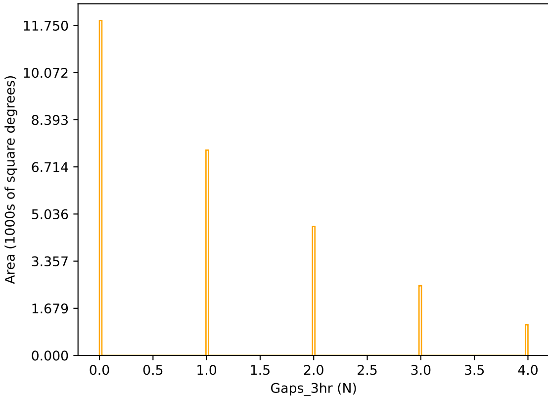
internal_u_expt27_nscale1.5v3.4_10yrs r band: Gaps_3hr
