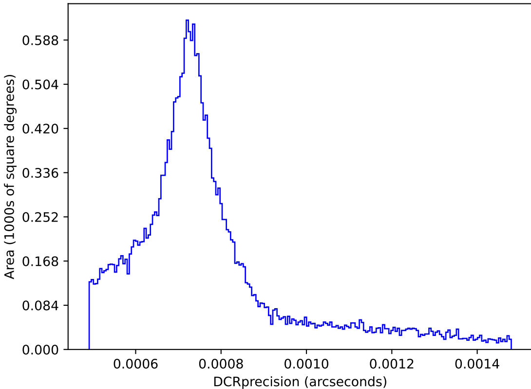
internal_u_expt27_nscale1.5v3.4_10yrs : DCRprecision
