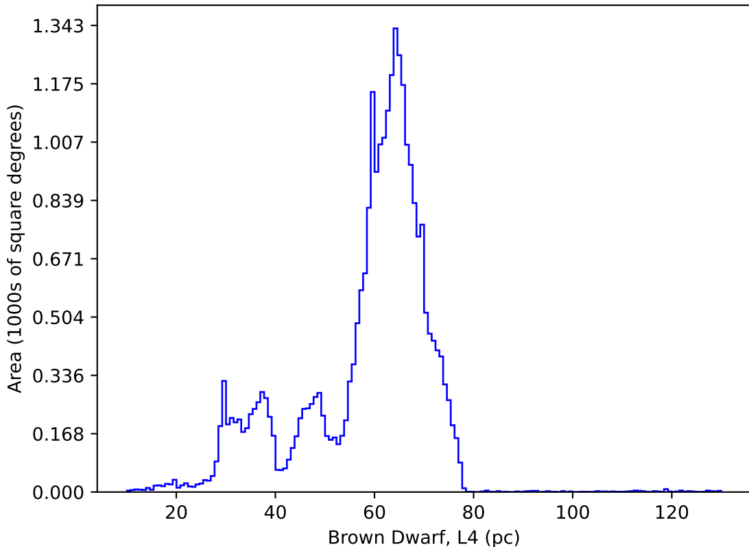
internal_u_expt27_nscale1.5v3.4_10yrs : Brown Dwarf, L4
