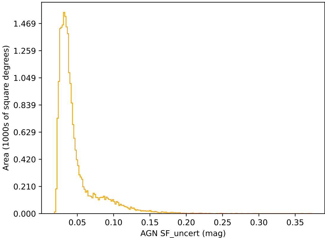
internal_u_expt27_nscale1.5v3.4_10yrs r band: AGN SF_uncert
