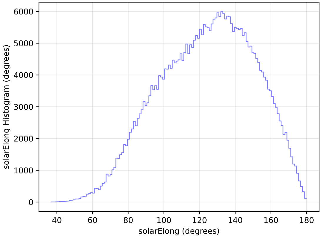
internal_u_expt27_nscale1.5v3.4_10yrs WFD y band: solarElong Histogram
