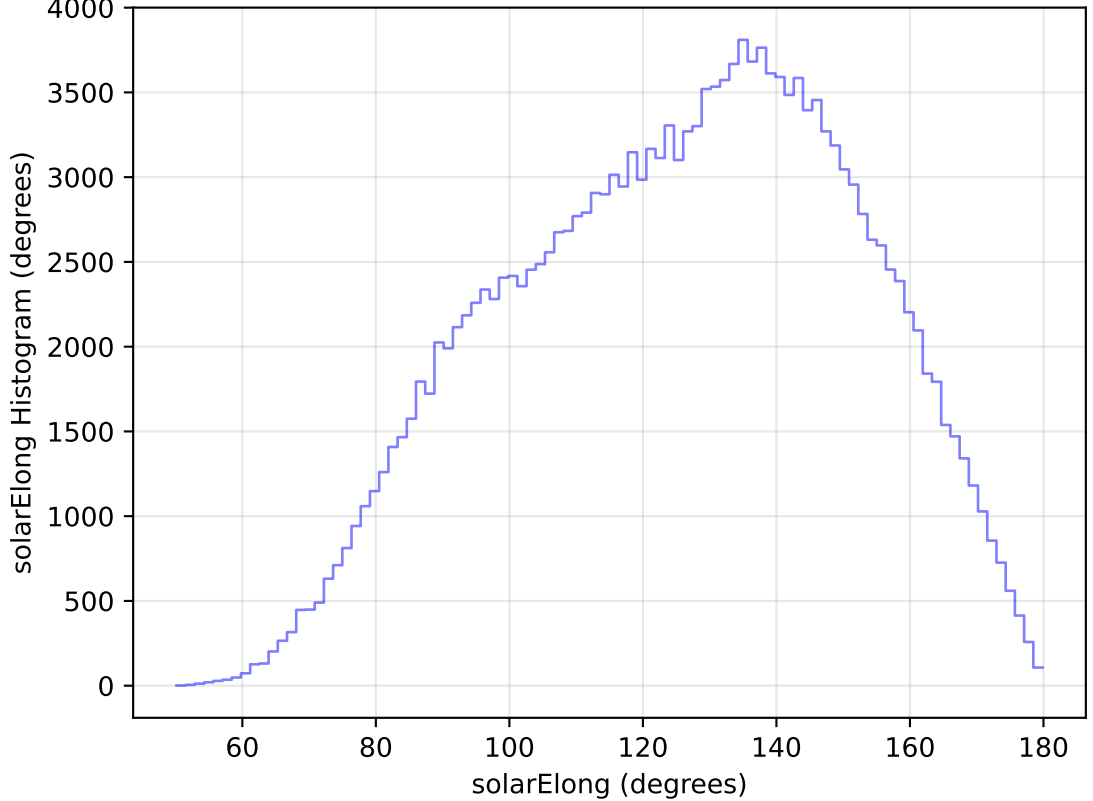
internal_u_expt27_nscale1.5v3.4_10yrs WFD u band: solarElong Histogram
