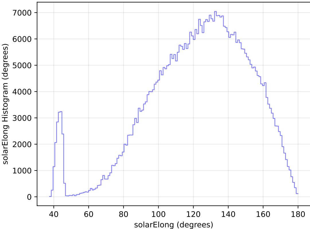
internal_u_expt27_nscale1.5v3.4_10yrs WFD r band: solarElong Histogram
