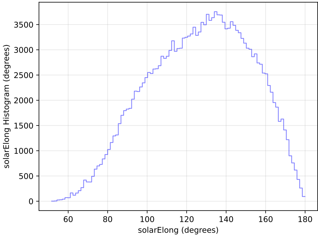
internal_u_expt27_nscale1.5v3.4_10yrs WFD g band: solarElong Histogram
