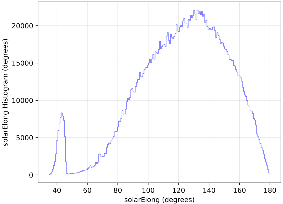
internal_u_expt27_nscale1.5v3.4_10yrs WFD all bands: solarElong Histogram
