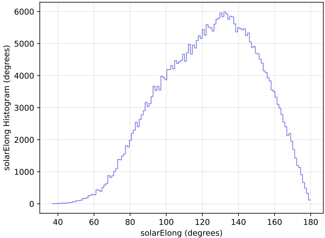
internal_u_expt27_nscale1.5v3.4_10yrs All sky y band: solarElong Histogram
