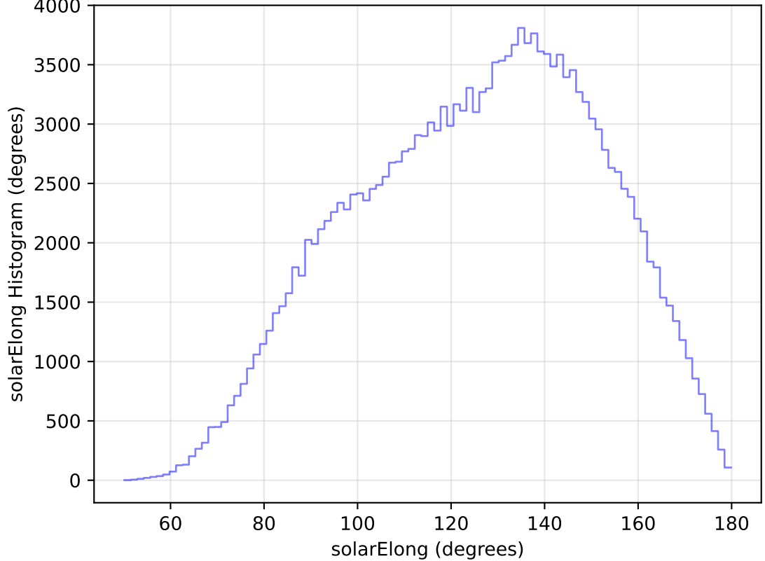
internal_u_expt27_nscale1.5v3.4_10yrs All sky u band: solarElong Histogram
