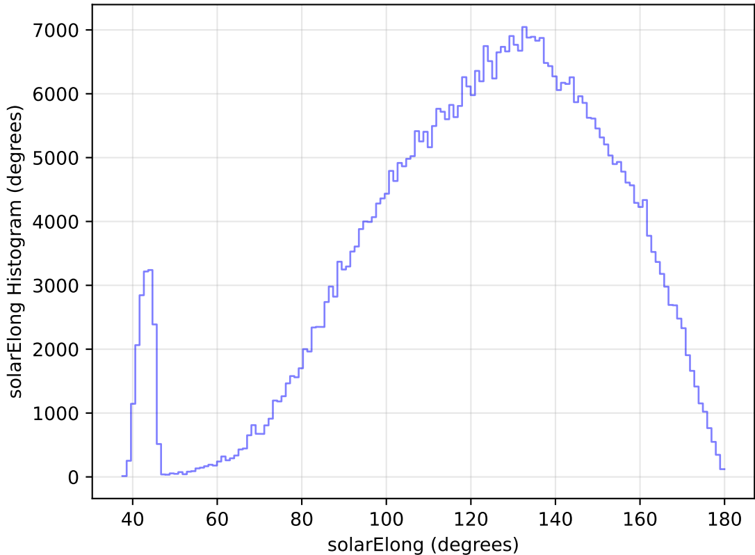
internal_u_expt27_nscale1.5v3.4_10yrs All sky r band: solarElong Histogram
