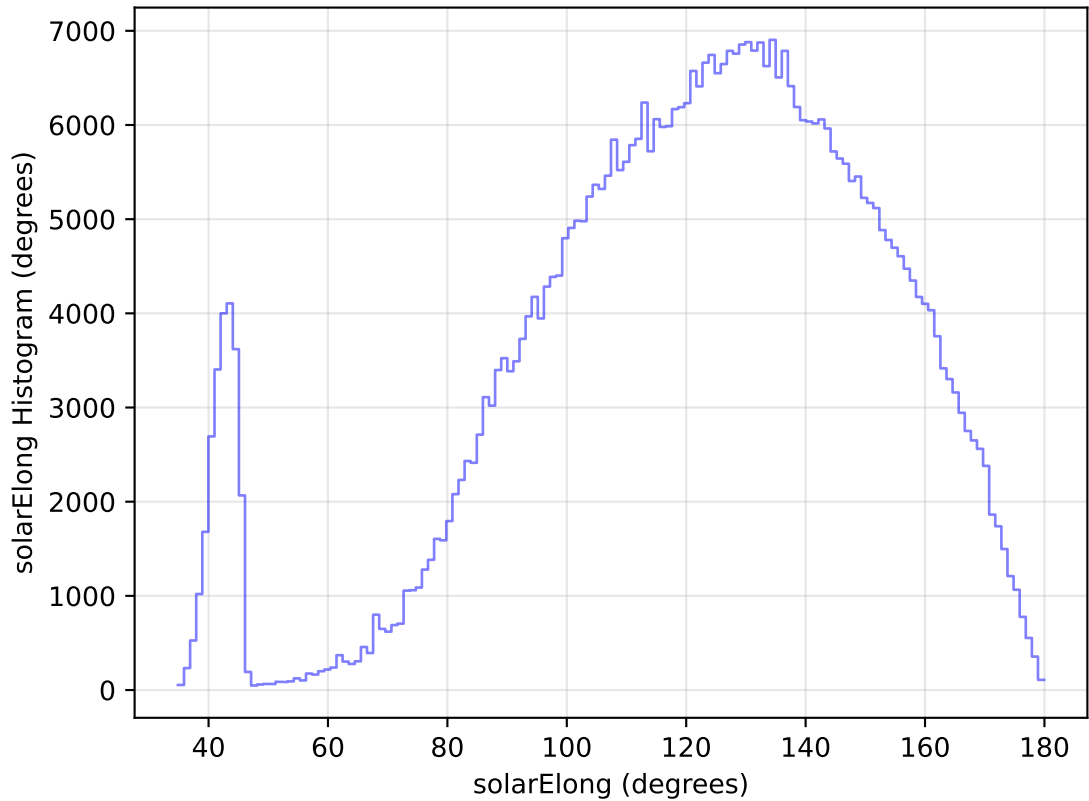
internal_u_expt27_nscale1.5v3.4_10yrs All sky i band: solarElong Histogram
