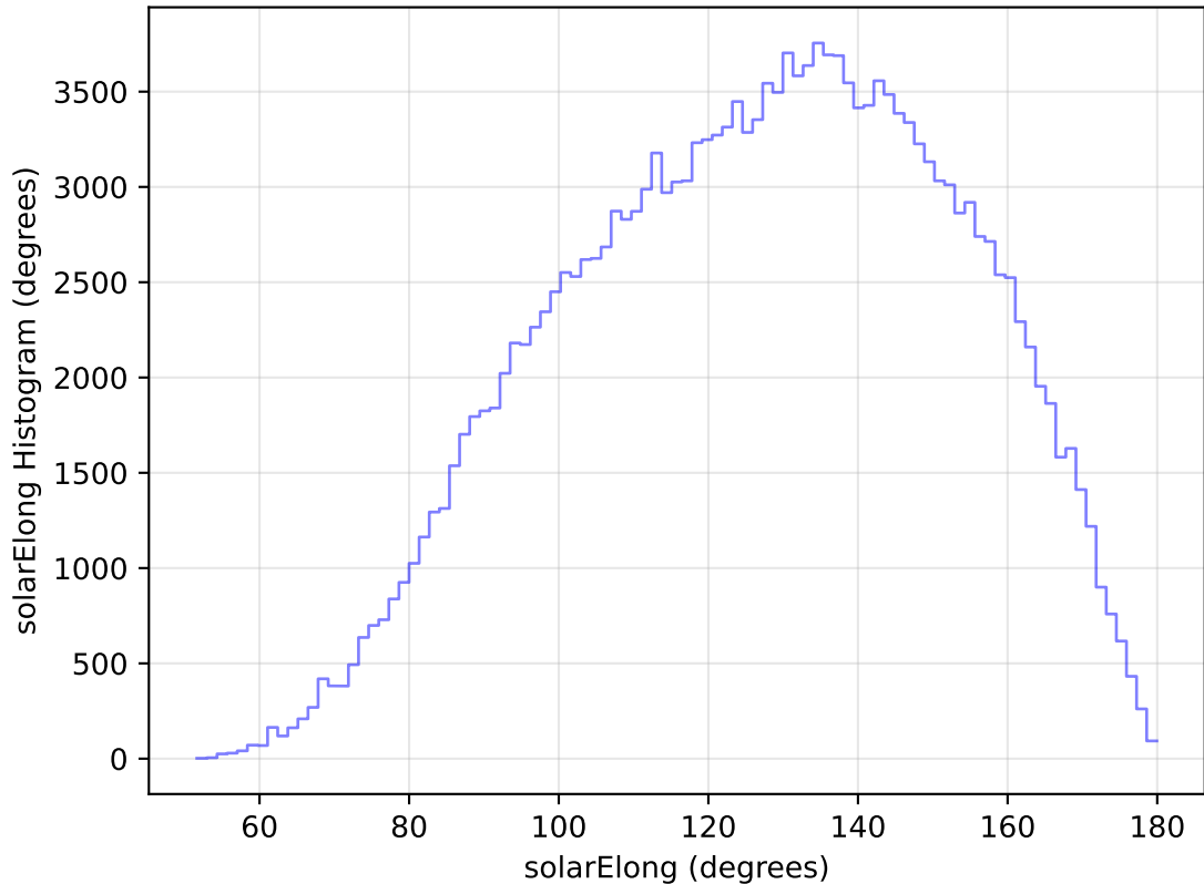
internal_u_expt27_nscale1.5v3.4_10yrs All sky g band: solarElong Histogram
