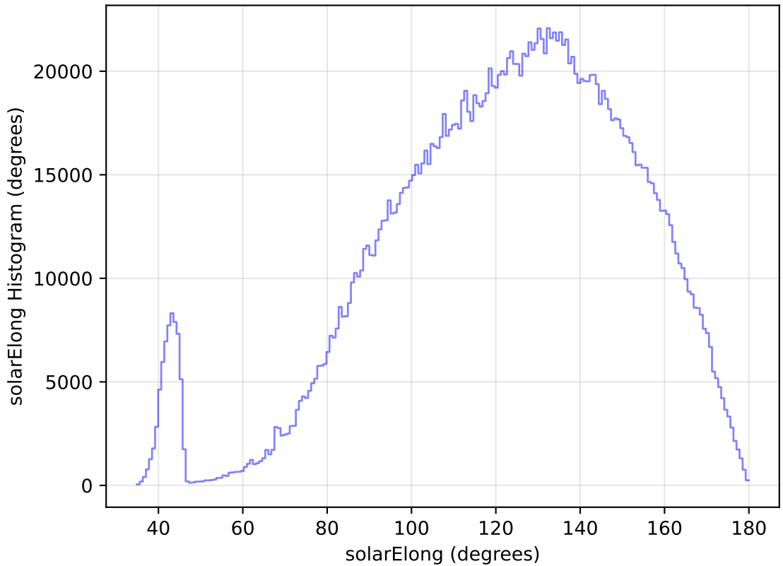
internal_u_expt27_nscale1.5v3.4_10yrs All sky all bands: solarElong Histogram
